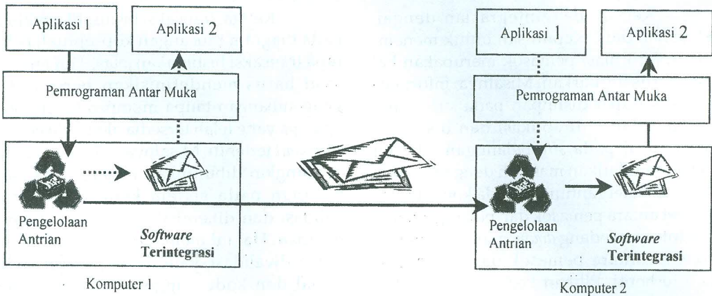
Gambar 6 Software Terintegrasi
